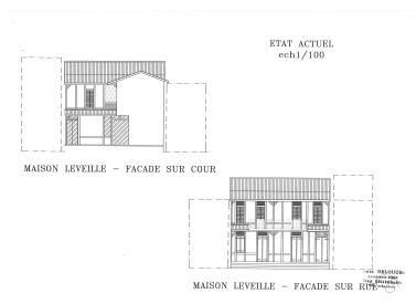
Relev  des fa ades, Sonia Delouche architecte, 2000. Phot. Sonia Delouche IVR03_202697300207NUCA
