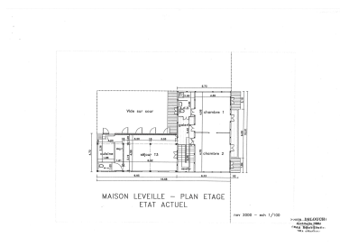
Plan de l' tage, Sonia Delouche architecte, 2000 Phot. Sonia Delouche IVR03_202697300204NUCA
